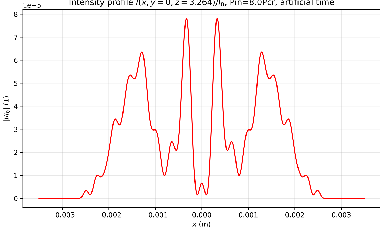
Intensity profile I(x, y = 0, z = 3.264)/I_0 , P_{in}=8.0P_{cr} , artificial time
